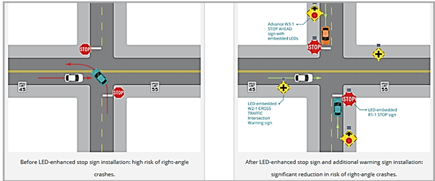
Depiction of current County rural intersection (left) and a proposed County rural intersection with improvements (right).
